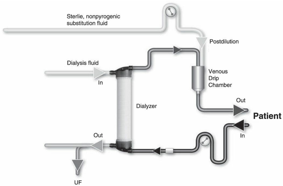
FIGURE 17.1 Postdilution online hemodiafiltration.
