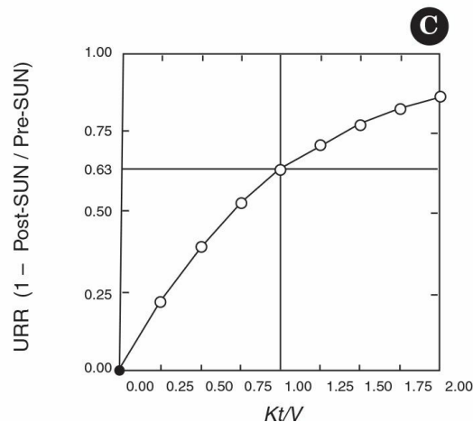
FIGURE 3.11 A: Another fixed-volume model, except this time the dialyzer outlet fluid is continually returned to the source tank throughout dialysis. As shown in B , the inlet SUN now falls exponentially during dialysis, reducing dialysis efficiency. C: With continuous outlet return, a URR of only 0.63 is reached when the total tank volume ( V ) is passed through the dialyzer, making Kt/V = 1.0 . (Reproduced from Daugirdas JT. Urea kinetic modeling. Hypertens Dial Clin Nephrol . Available at: http://www.hdcn.com .)
