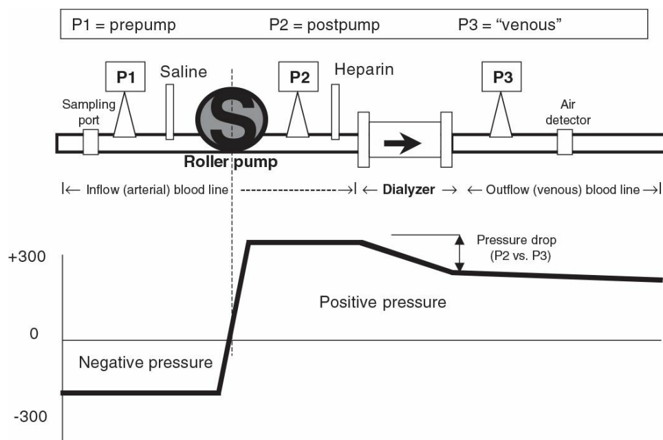
FIGURE 4.1 Pressure monitors (P1, P2, and P3) and pressures in blood circuit.
