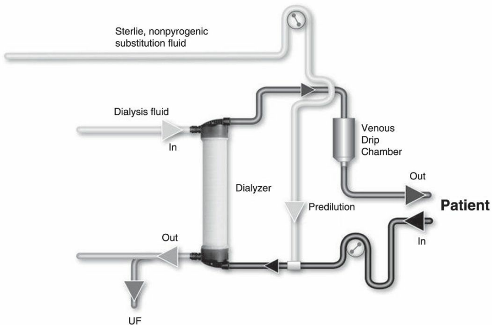
FIGURE 17.2 Predilution online hemodiafiltration.
