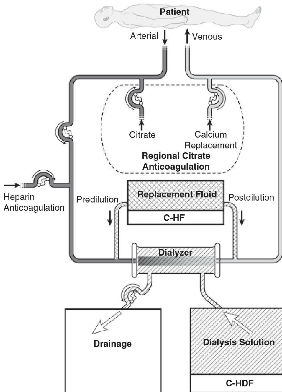
FIGURE 15.2 Typical circuit for continuous hemofiltration and slow continuous hemodiafiltration. In slow continuous hemofiltration (C-HF), replacement fluid can be infused in the predilution mode, or postdilution mode, or both simultaneously. In slow continuous hemodiafiltration, hemodialysis is performed concurrently with C-HF. Anticoagulation with either heparin or regional citrate is shown.
